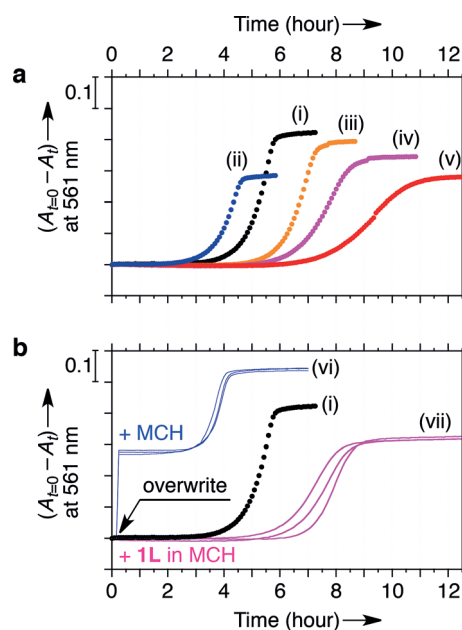
Figure 4. a) Time profile of transformation from J- to H-aggregates: i) [1M] = 50 \mu M , ii) [1M] = 35 \mu M , iii) [1M] = 45 \mu M , [1L] = 5 \mu M , iv) [1M] = 40 \mu M , [1L] = 10 \mu M , and v) [1M] = 35 \mu M , [1L] = 15 \mu M . b) Designated t_{50} value of conditions (i) and (vi) was advanced and (vii) delayed by the addition of pure MCH and 1L solution, respectively, 10 min after the measurement was started. Each overwriting experiment was reproduced three times. The final concentrations of the porphyrin molecules were (vi) [1M] = 35 \mu M , and (vii) [1M] = 40 \mu M , [1L] = 10 \mu M . During the measurements, the solution was stirred at 400 rpm at 308 K.
