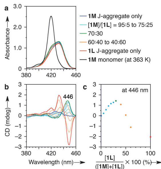
Figure 3. a) Absorption and b) CD spectra of the 1M/1L mixtures. c) Plot of the CD intensity at 446 nm as a function of the 1M/1L ratio. [\textbf{1M}] + [\textbf{1L}] = 50 \mu\text{M} .
